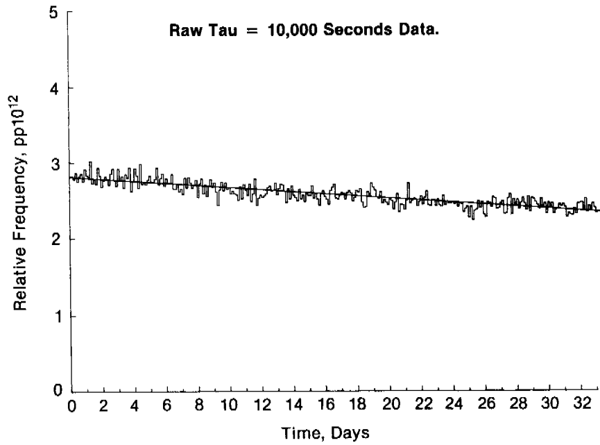
Figure 6. EG&G GPS RFS Prototype No. 2 stability test, 6/16/83-7/19/83.
