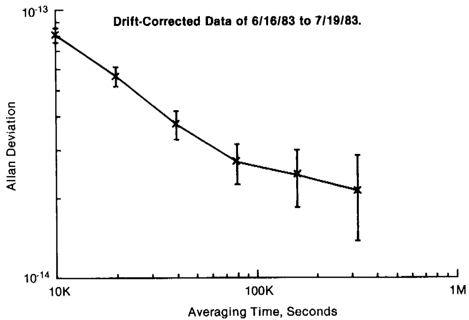
Figure 6. EG&G GPS RFS Prototype No. 2 stability test, 6/16/83-7/19/83.
