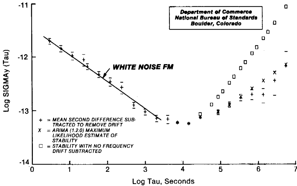
Figure 5. EG&G RB versus NBS ensemble.
